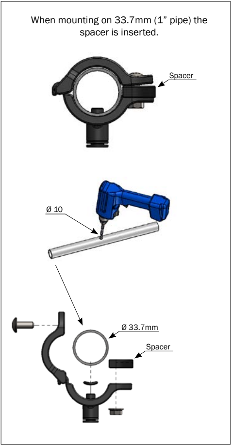
Mounting with master drill clamp (61195)
