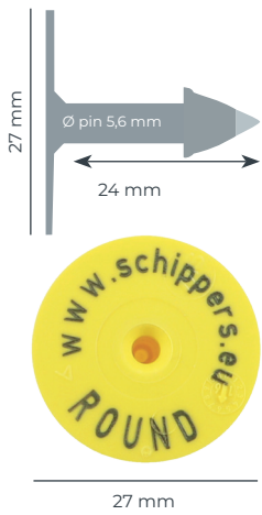
MS Tag Round (Robust pin)
