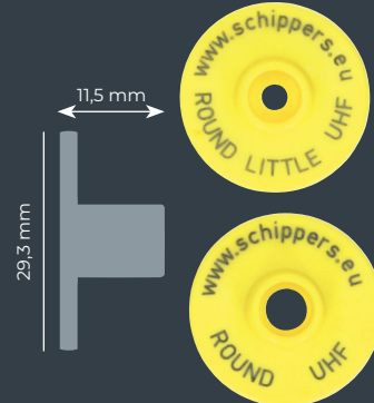
MS Tag Round UHF (Open)
