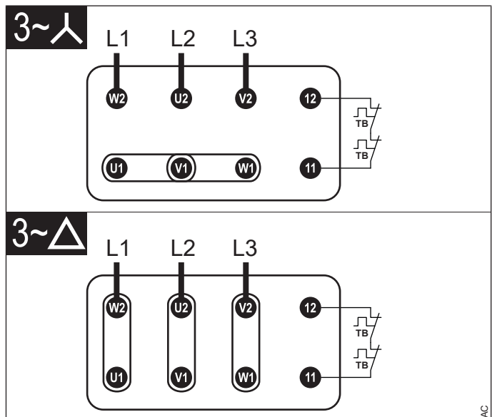
Illustration 4: 3~ STAR / DELTA with optional thermal detectors (thermostats)
