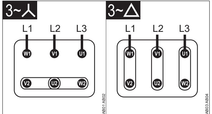
Illustration 3: 3~ STAR / DELTA (standard terminal block)
