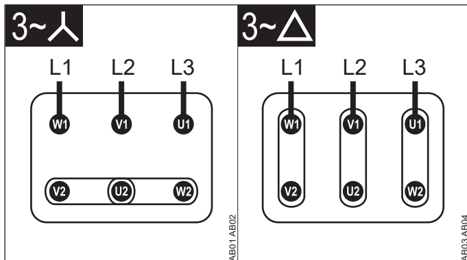
Fig. 3: 3~ ETOILE / TRIANGLE (bloc terminal standard)
